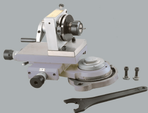
ER Collet Divider Punch Grinder Attachment
